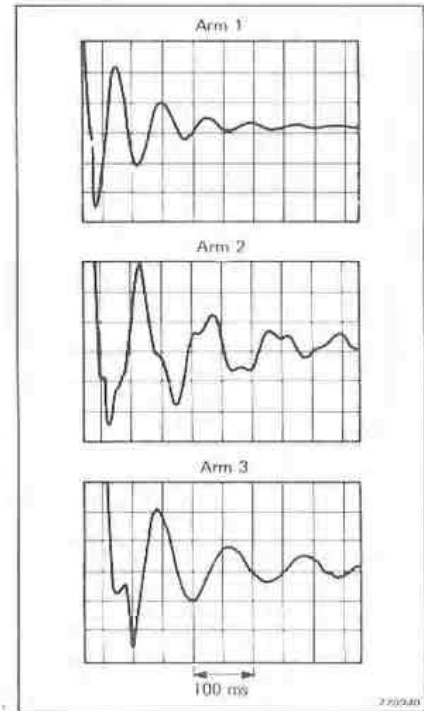
Fig.25. Oscillograms of the transient test using the record mentioned in Fig.24. Each picture shows the voltage from the cartridge reflecting the oscillations initiated by the step. As seen in most of the examples the oscillations continue for more than 0,5 s (1/4 revolution of the record)
