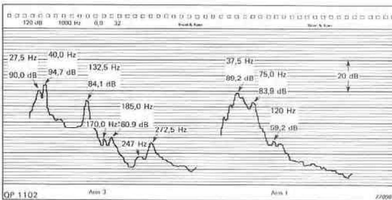
Fig.35. Frequency and level of resonant modes in a turntable with two different arms
