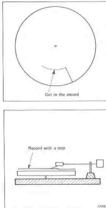
Fig.24. A small cut in a record enables the two parts to be displaced a bit. A well-defined step is then obtained for transient tests of cartridge/arm combinations
