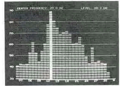
Fig.34. Spectra from the three different arms with the cartridge resting on a non-rotating record when exposed to broadband pink noise. Set up: see Fig.32
