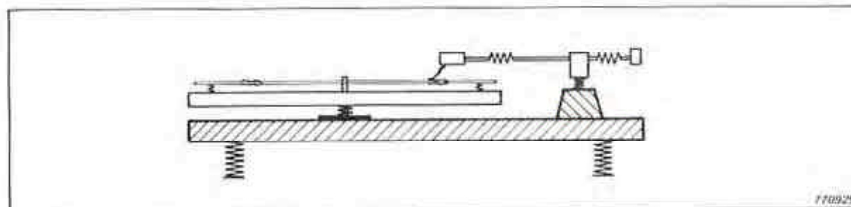
Fig.1. Sketch of the placement of elastic couplings between the various parts in a turntable. The compliance of these couplings builds up resonances which disturbs the relative position between the cartridge needle and the record groove. This results in deterioration of the sound quality
