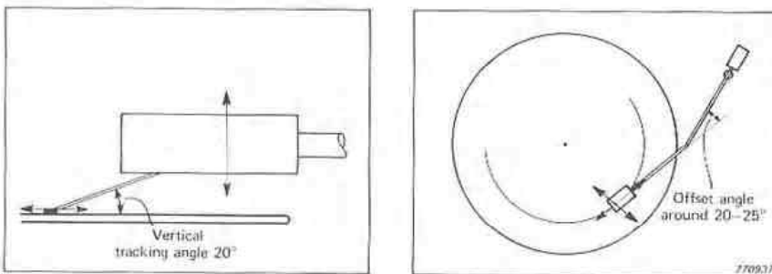
Fig. 20. Left: Oscillations of the tonearm at the arm resonance in the vertical plane causes wow and flutter proportional to the vertical tracking angle Right: Oscillations in the horizontal plane increases wow and flutter proportional to the offset angle. (Note that parallel tracking arms have an offset angle of zero degree and gives therefore superior wow specification)
