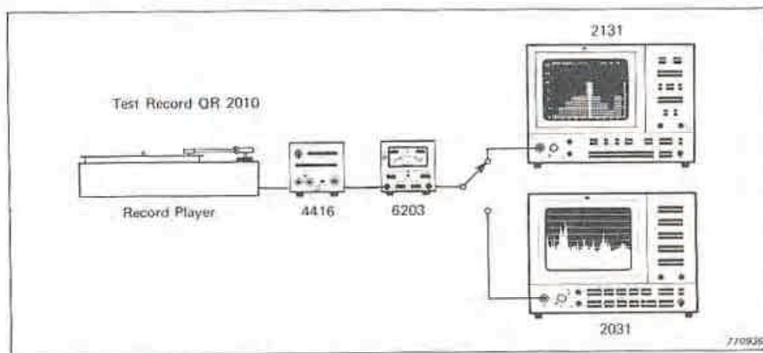
Fig.17. A sophisticated version for flutter analysis using B & K Type 2131 or B & K Type 2031
