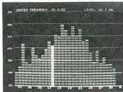
Fig.34. Spectra from the three different arms with the cartridge resting on a non-rotating record when exposed to broadband pink noise. Set up: see Fig.32
