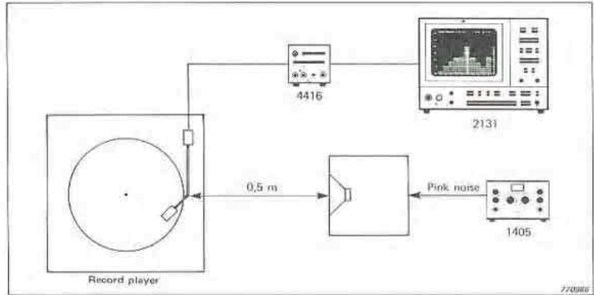
Fig.32. Measurement of the resonance modes in a turntable, when exposed to mixed acoustical-mechanical excitation. The signal fed to the loudspeaker is broadband pink noise
