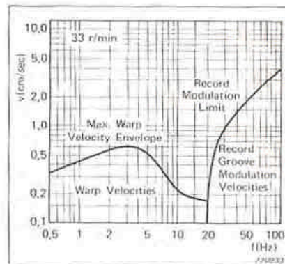
Fig.7. Velocity spectrum of phonograph records
