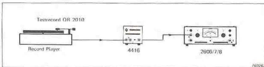
Fig.5. Basic set-up for measuring rumble in a turntable
