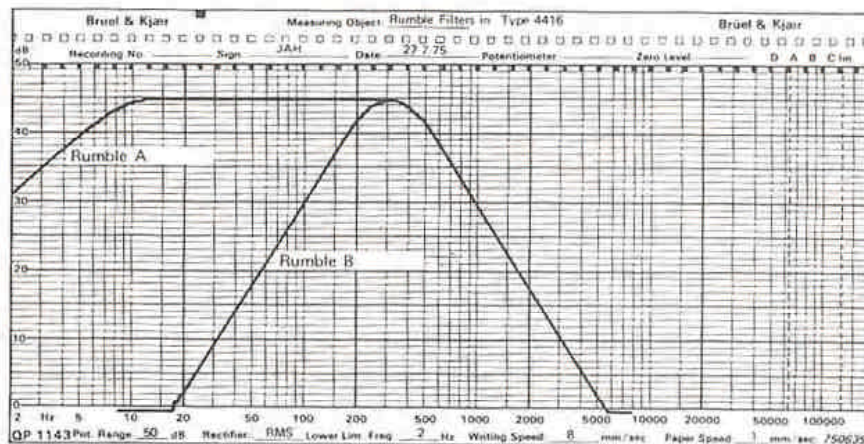
Fig.6. Standard weighting networks A and B for rumble measurements
