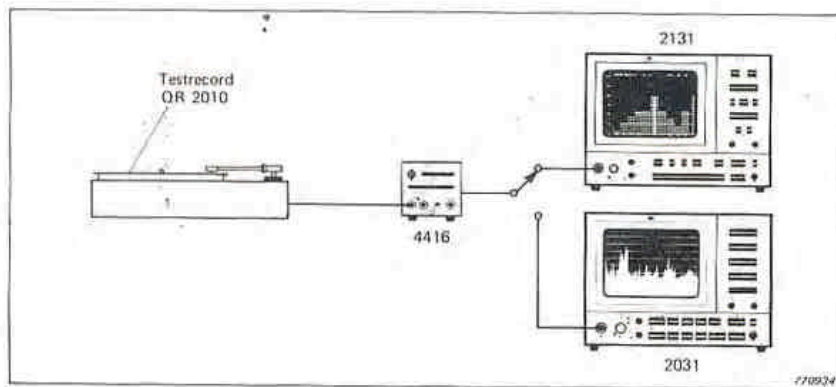
Fig.13. Set-up for measurement of rumble using Parallel Analyzers B & K Type 2031 or 2131
